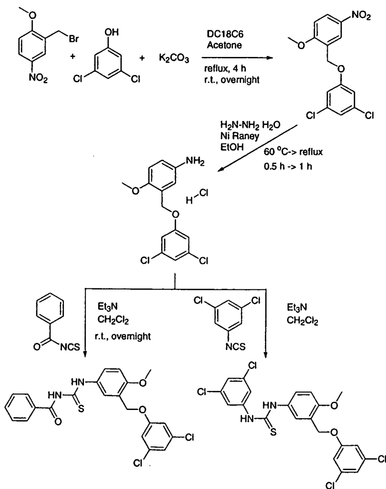
Scheme VIII
